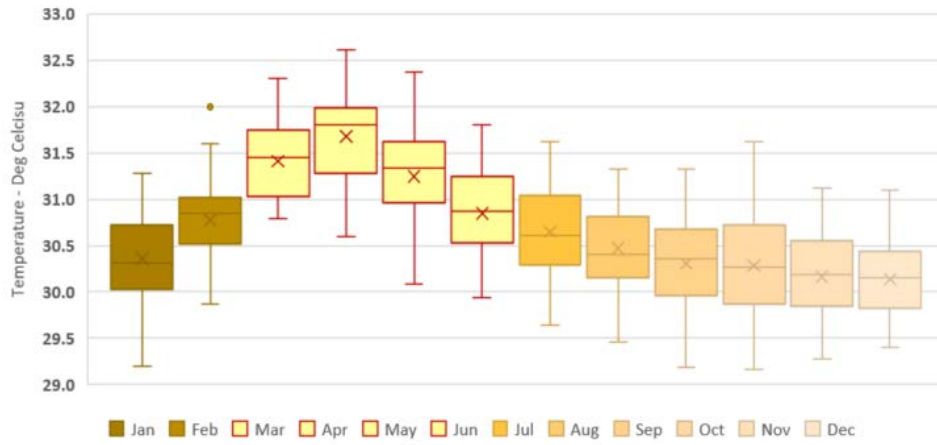
Average Daily Maximum Temperature by month
