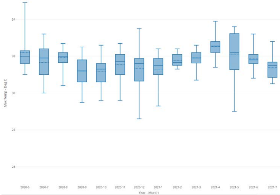
(Jun 2020 to Jul 2021)' Max Temperature for Hulhule'
