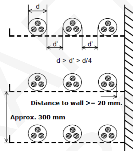
Figure 9 – Scheme of distribution of the MV cables separated less than a diameter lying on a perforated tray in open air installations and reference distances considered
