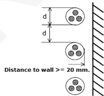
Figure 6 – Scheme of MV cables lying on structures or walls in open air installations and reference distances considered
