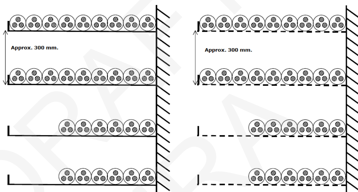
Figure 7 – Scheme of MV cables in contact between them and with the wall lying on trays in open air installations and reference distances considered
